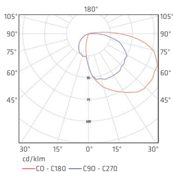
OPTIMA 2 1x40W
