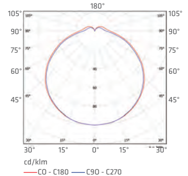
PHOBOS RCR 2x23W
